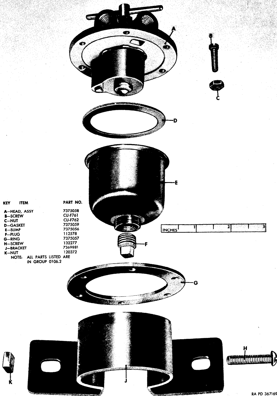
Figure 01-13. Oil filter, assy (7375060) (Cuno)—exploded view
