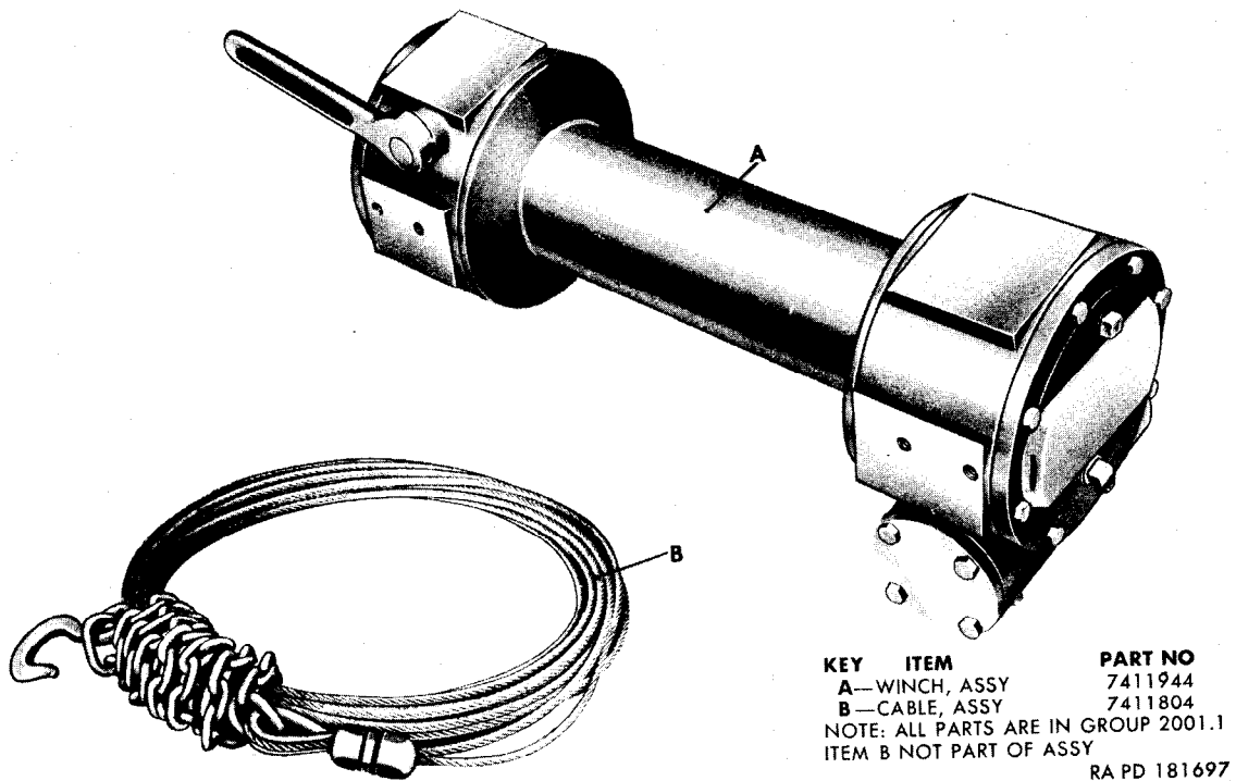
Figure 20-2. Winch, assy and related parts
