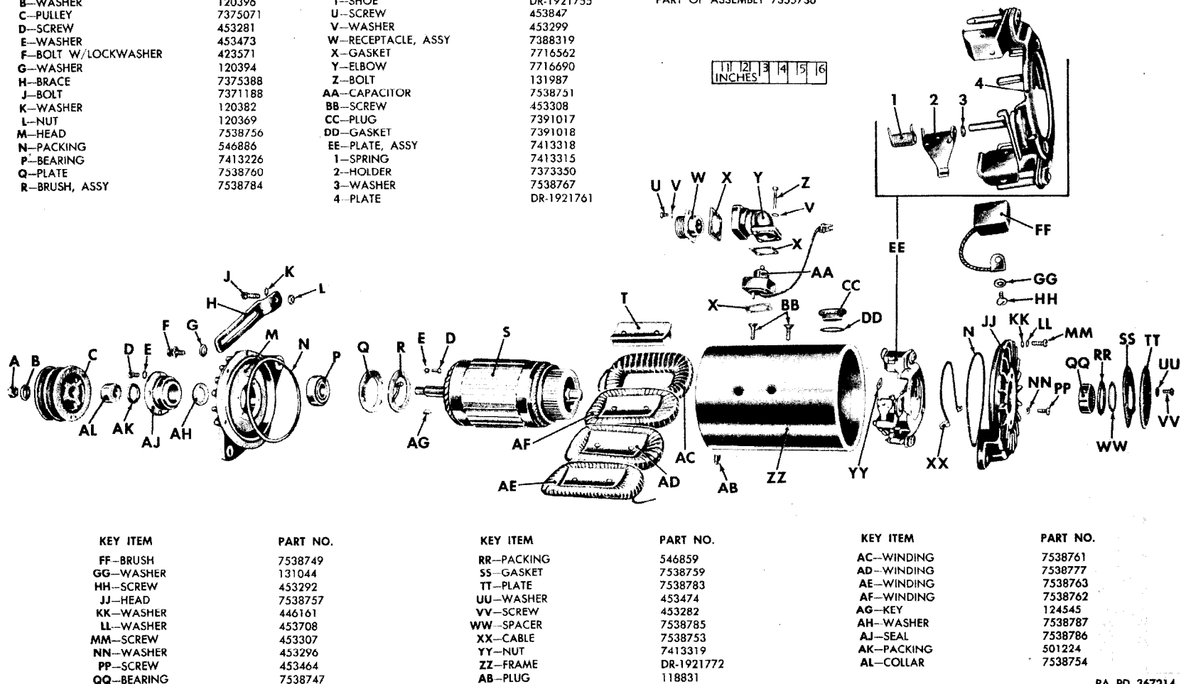
Figure 06-2. Generator, assy (7355736) Delco-Remy, 24-volt—exploded view
