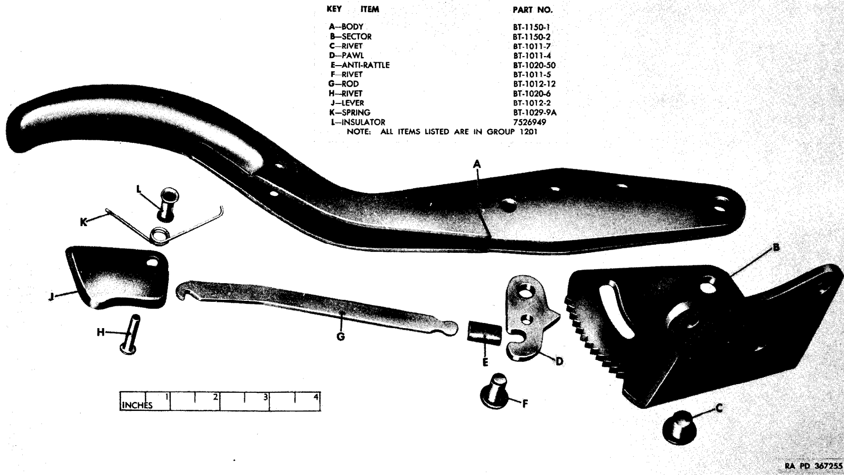
Figure 12-1. Handle, hand brake, assy (8329628)—exploded view
