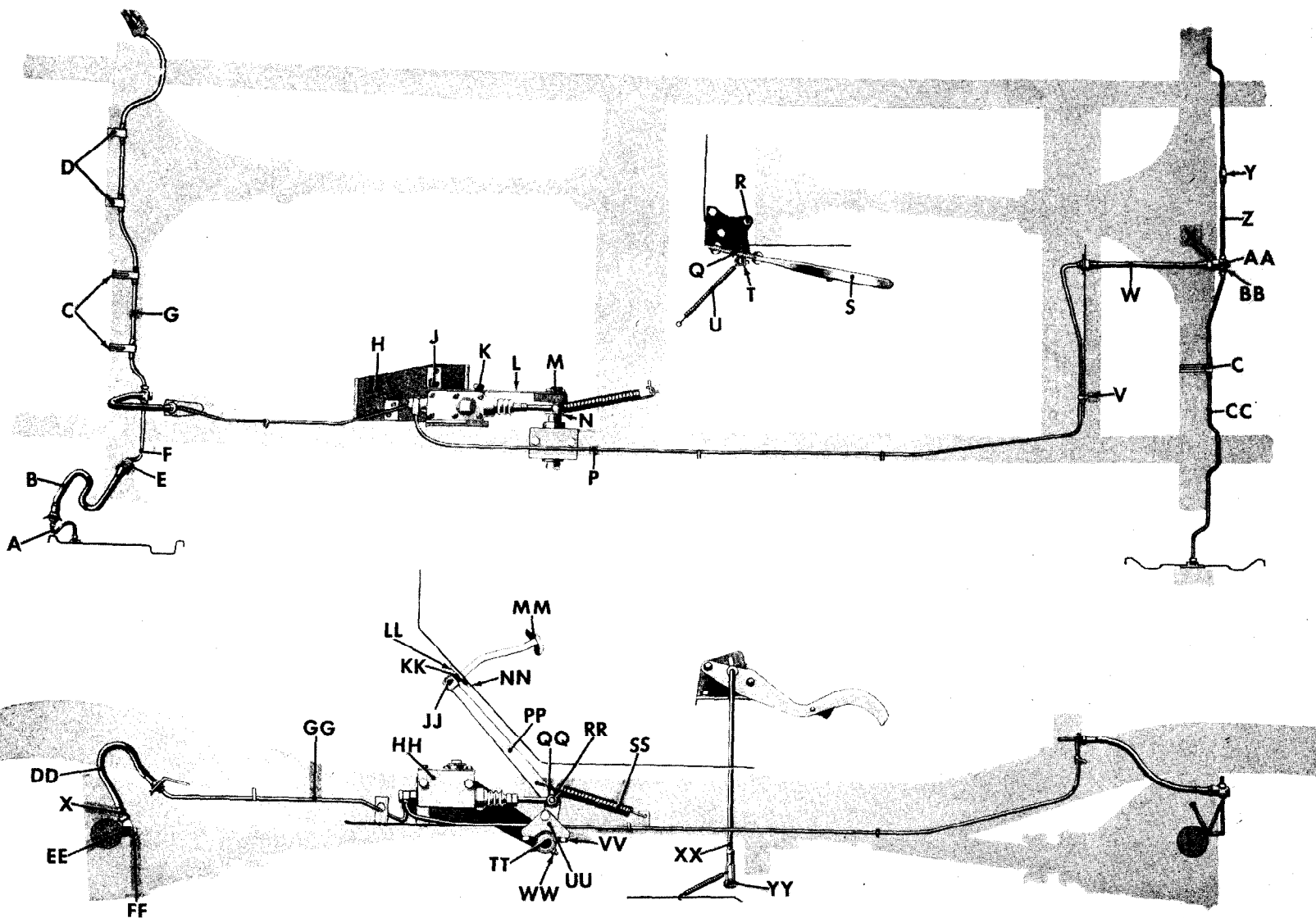
Figure 12-7. Brake system
