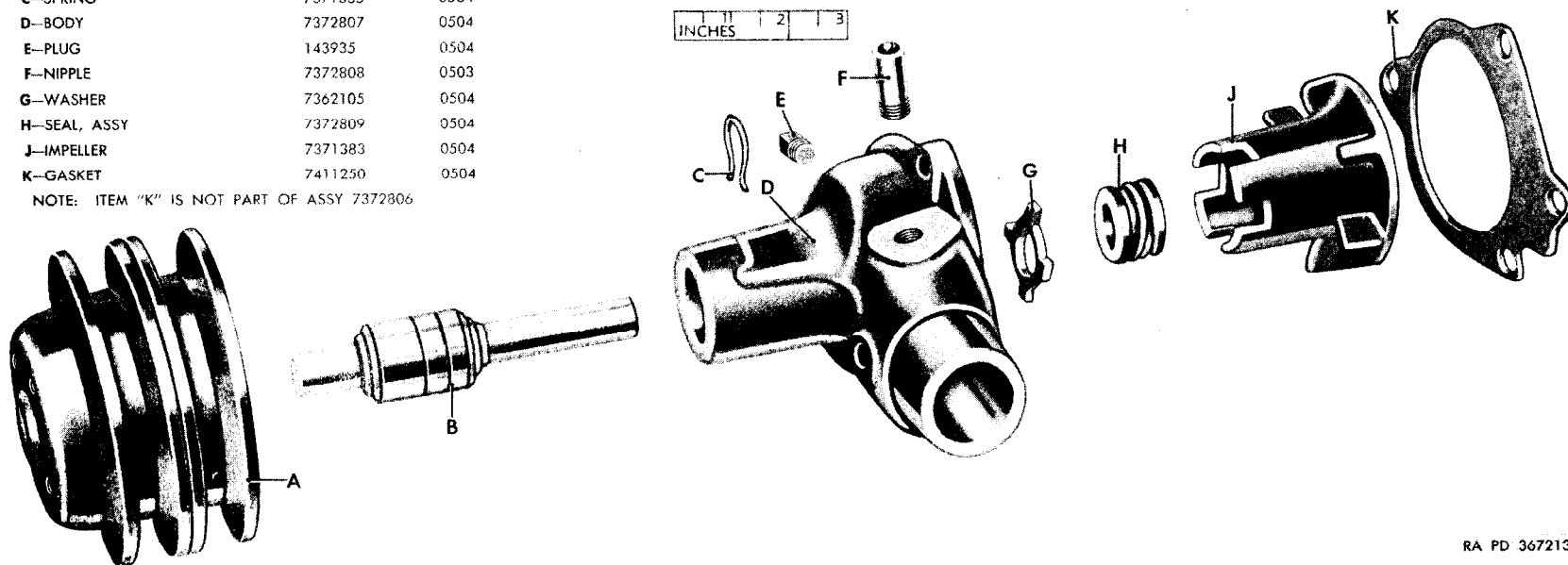
Figure 05-2. Water pump, assy (7372806)—exploded view
