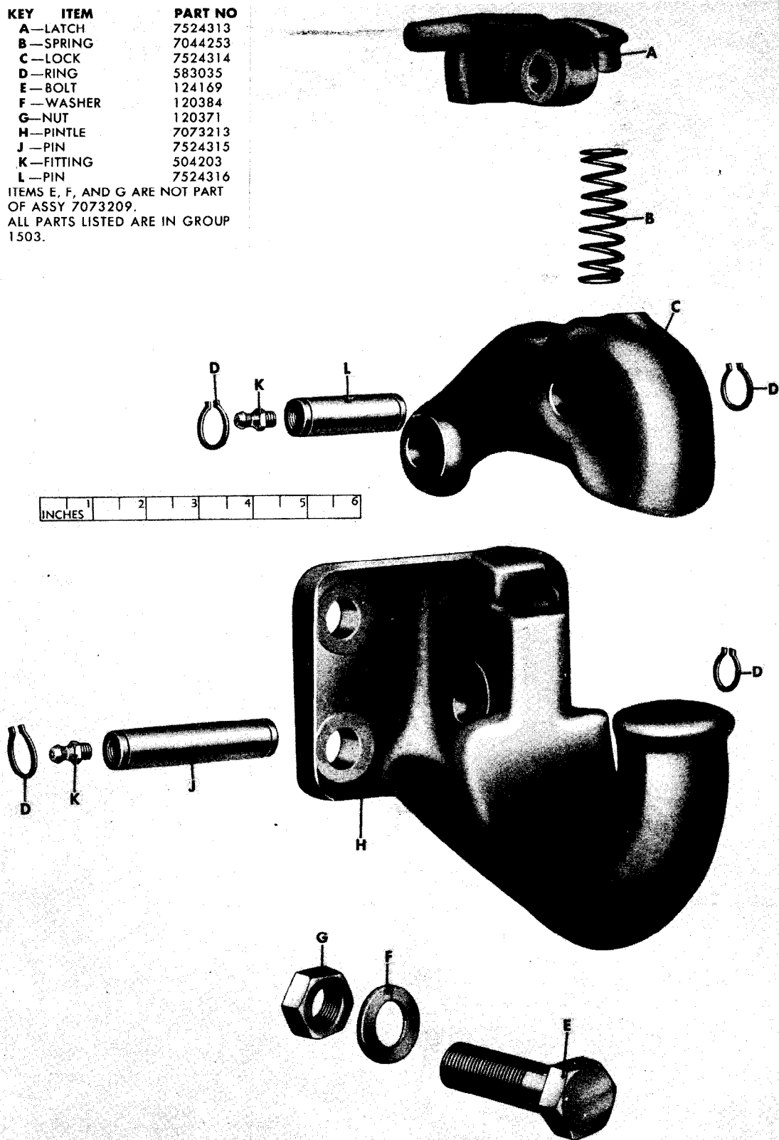
Figure 15-2. Pinle hook, assy (7073209)—exploded view
