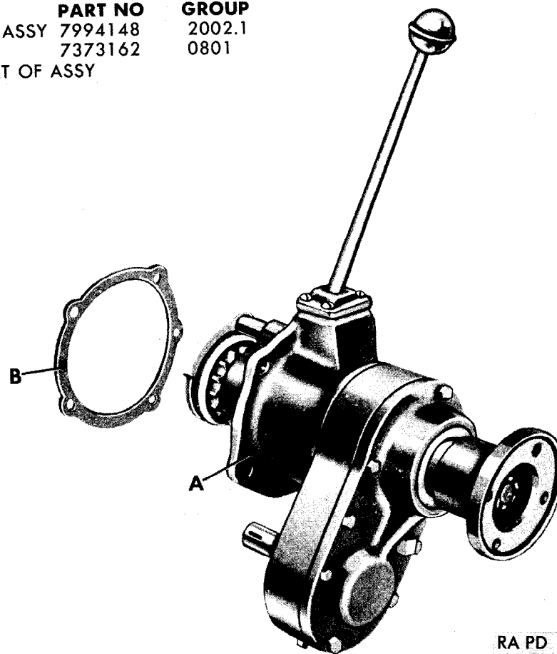
Figure 20-5. Power-take-off (7994148) and related parts
