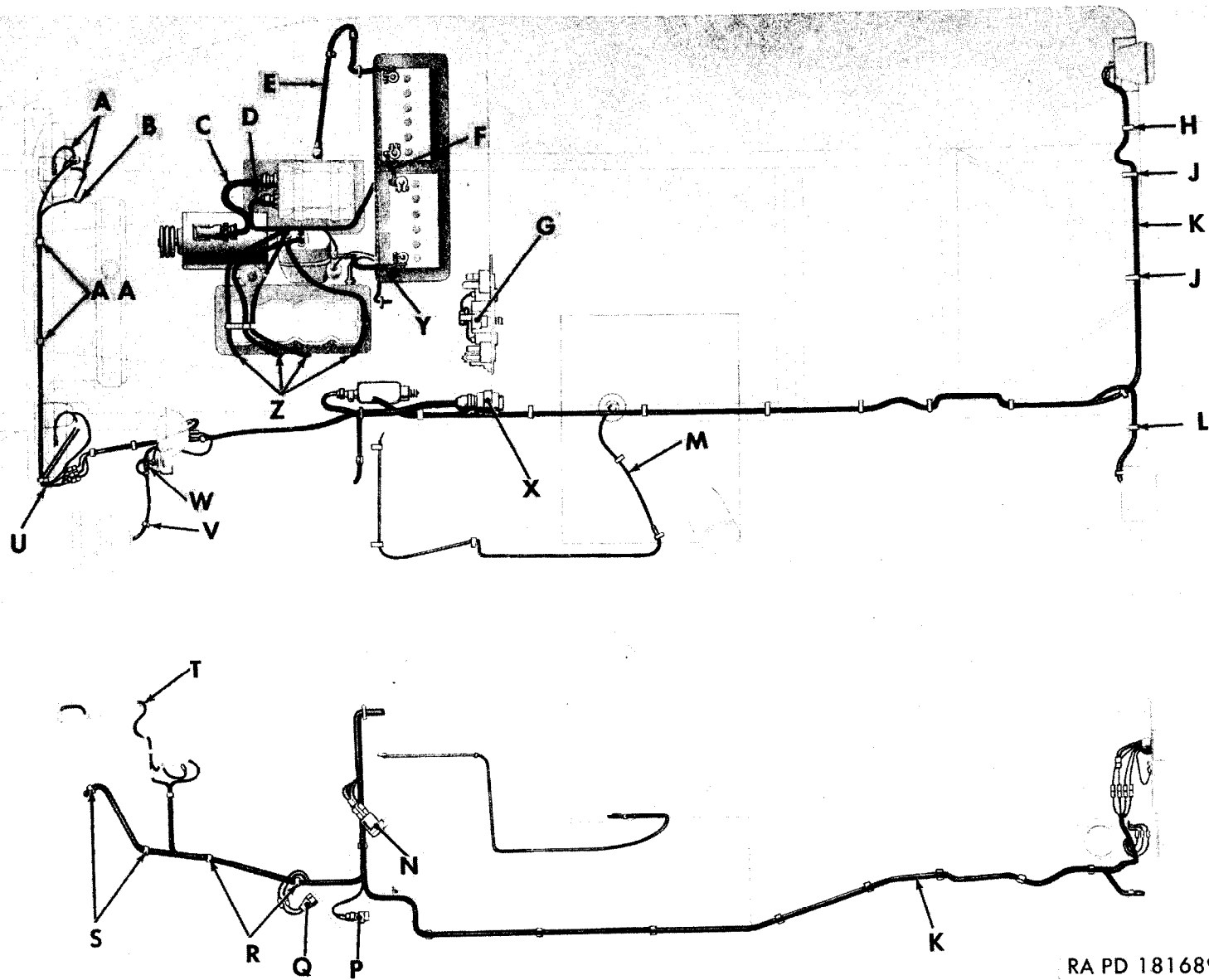
Figure 06-11. Wiring system
