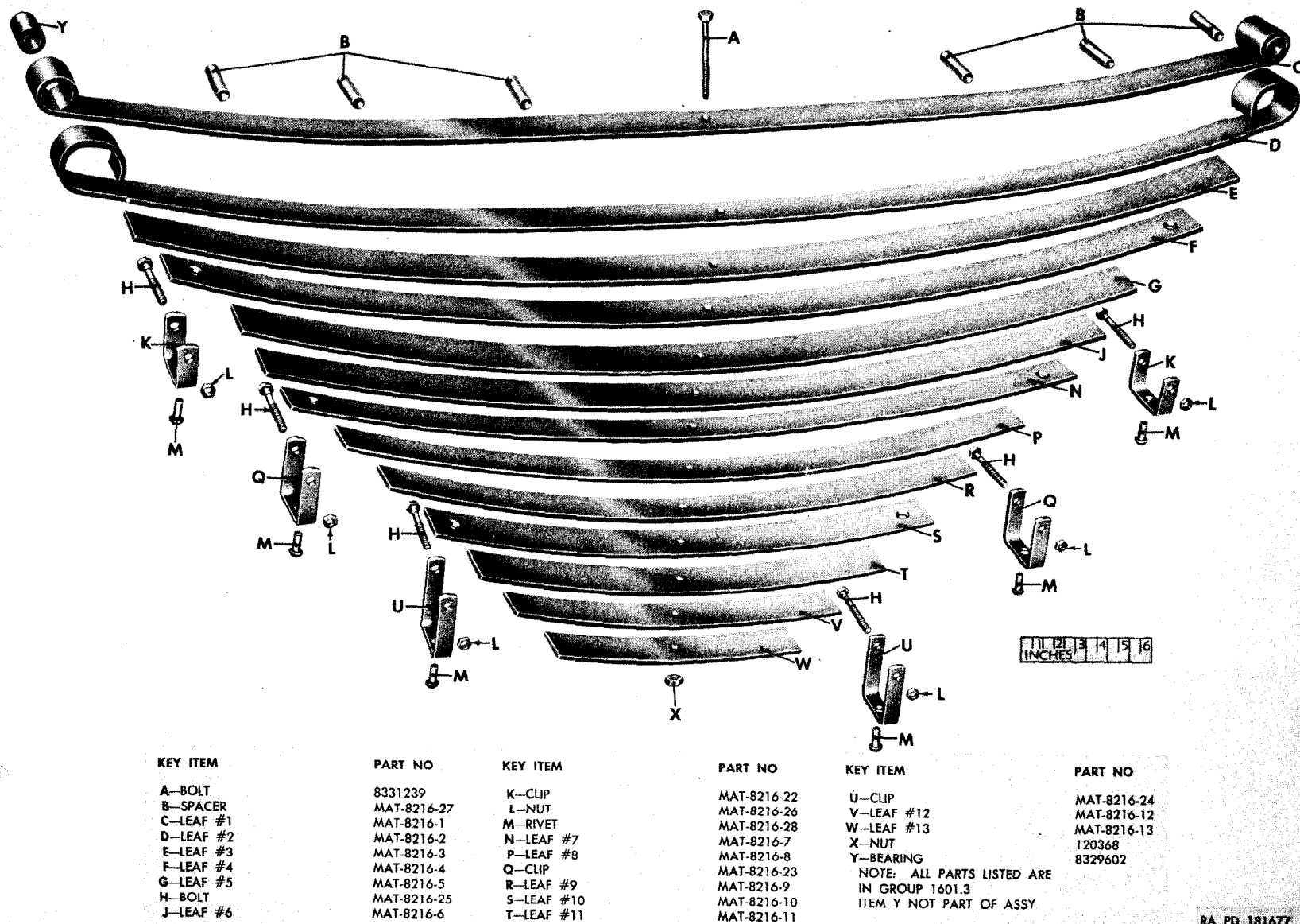
Figure 16-6. Rear spring, assy (8330508)—exploded view
