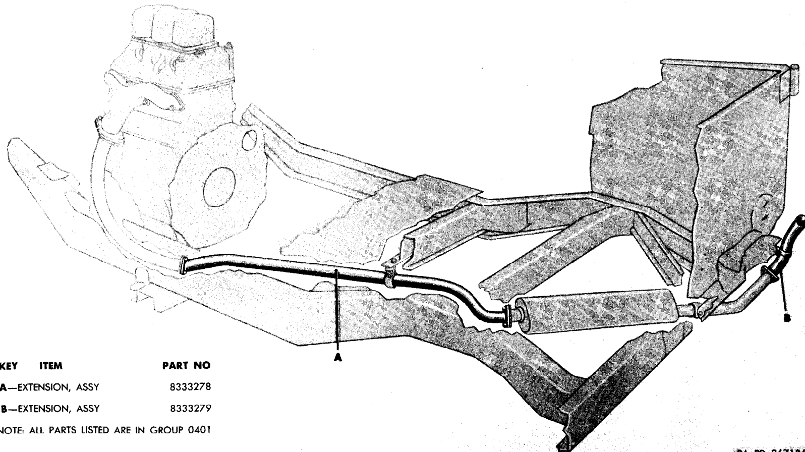
Figure 04-2. Exhaust system (M170)
