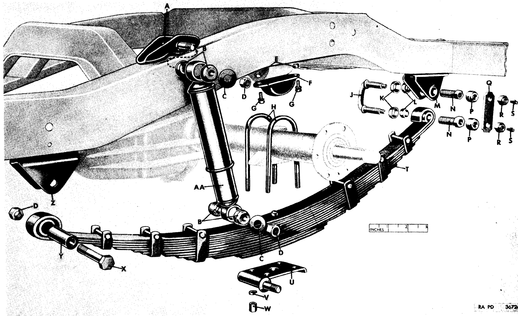
Figure 16-2. Rear spring and shock absorber
