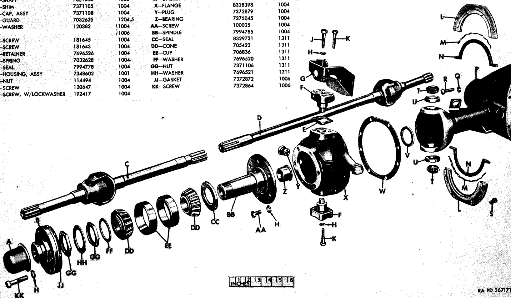
Figure 10-4. Steering knuckle and universal joint—exploded view
