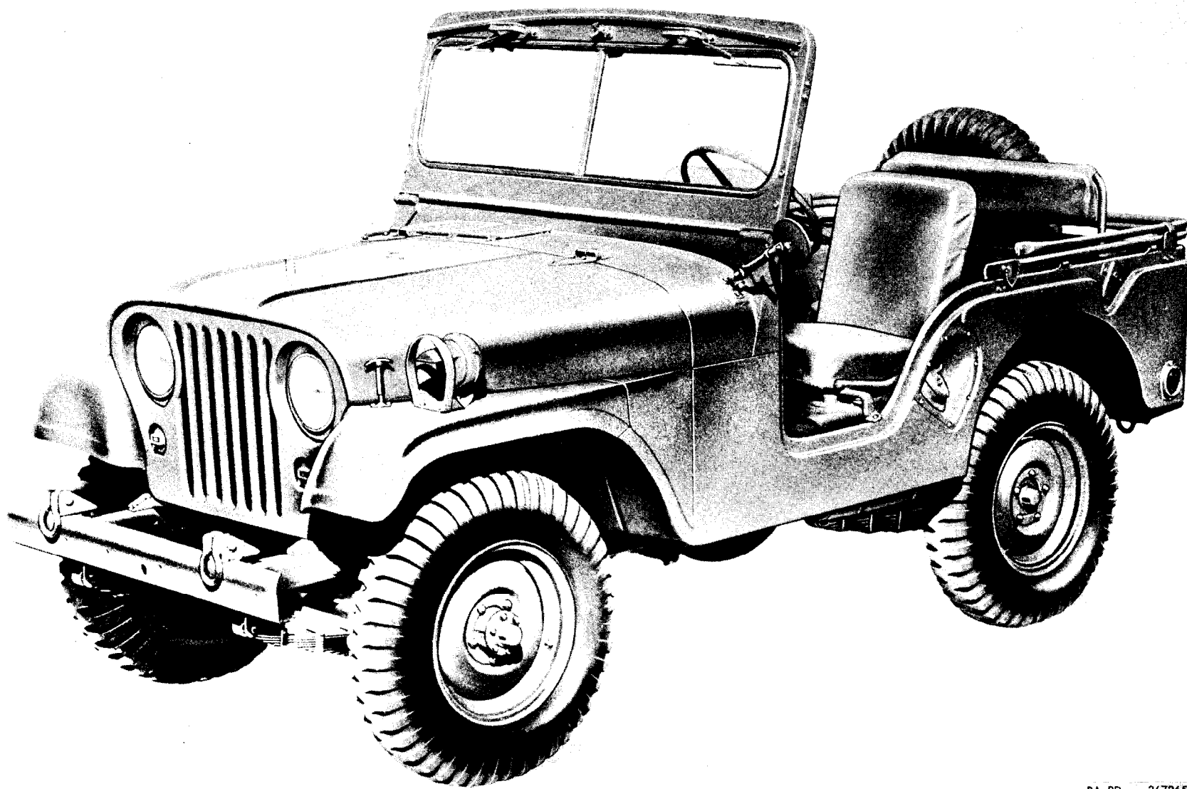
Figure 3. Truck, Utility: \frac{1}{4} -ton, 4 x 4, M38A1—left front view, top down
