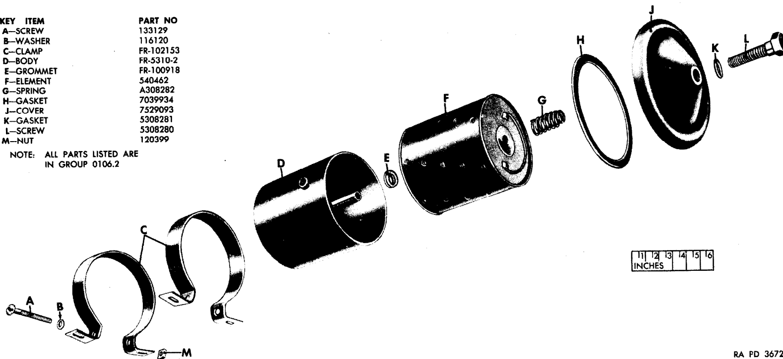
Figure 01-12. Oil filter, assy (540501) (Fram)—exploded view
