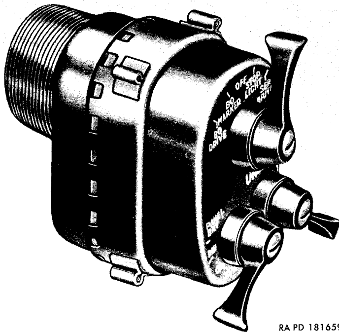
Figure 06-8. Light switch (7368702)
