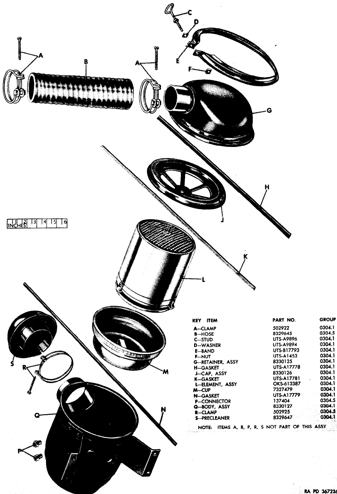
Figure 03-6. Air cleaner, assy (8329642)—exploded view
