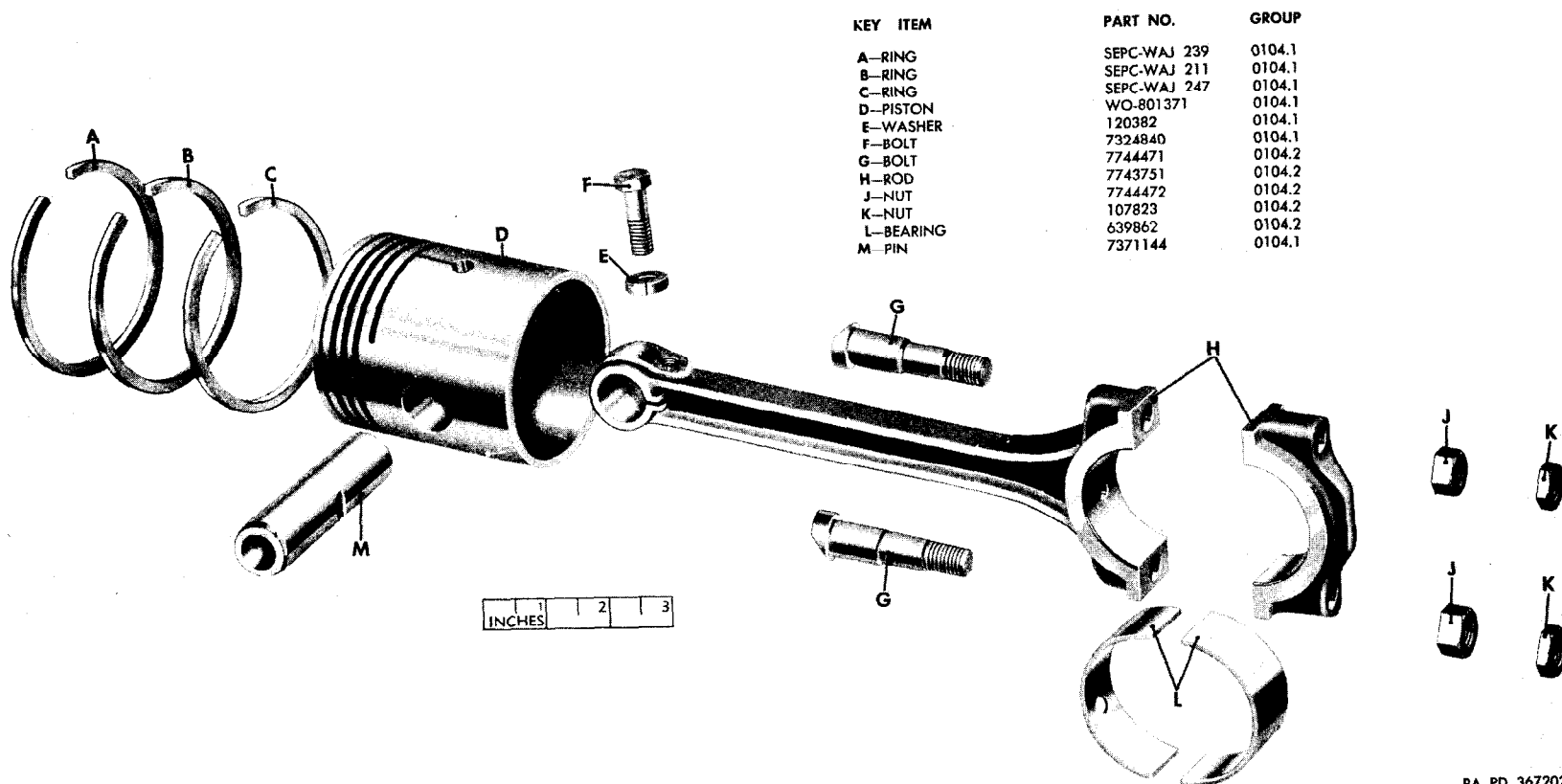
Figure 01-8. Piston and connecting rod—exploded view
