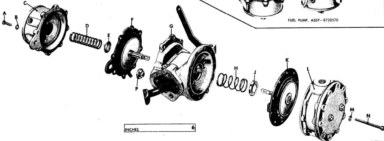
Figure 03-2. Fuel and vacuum pump, assy (8720570)—exploded view
