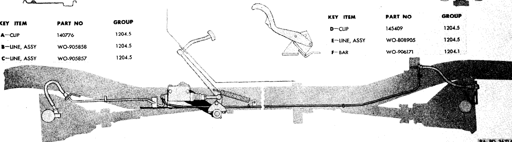
Figure 12-8. Brake system (M170)
