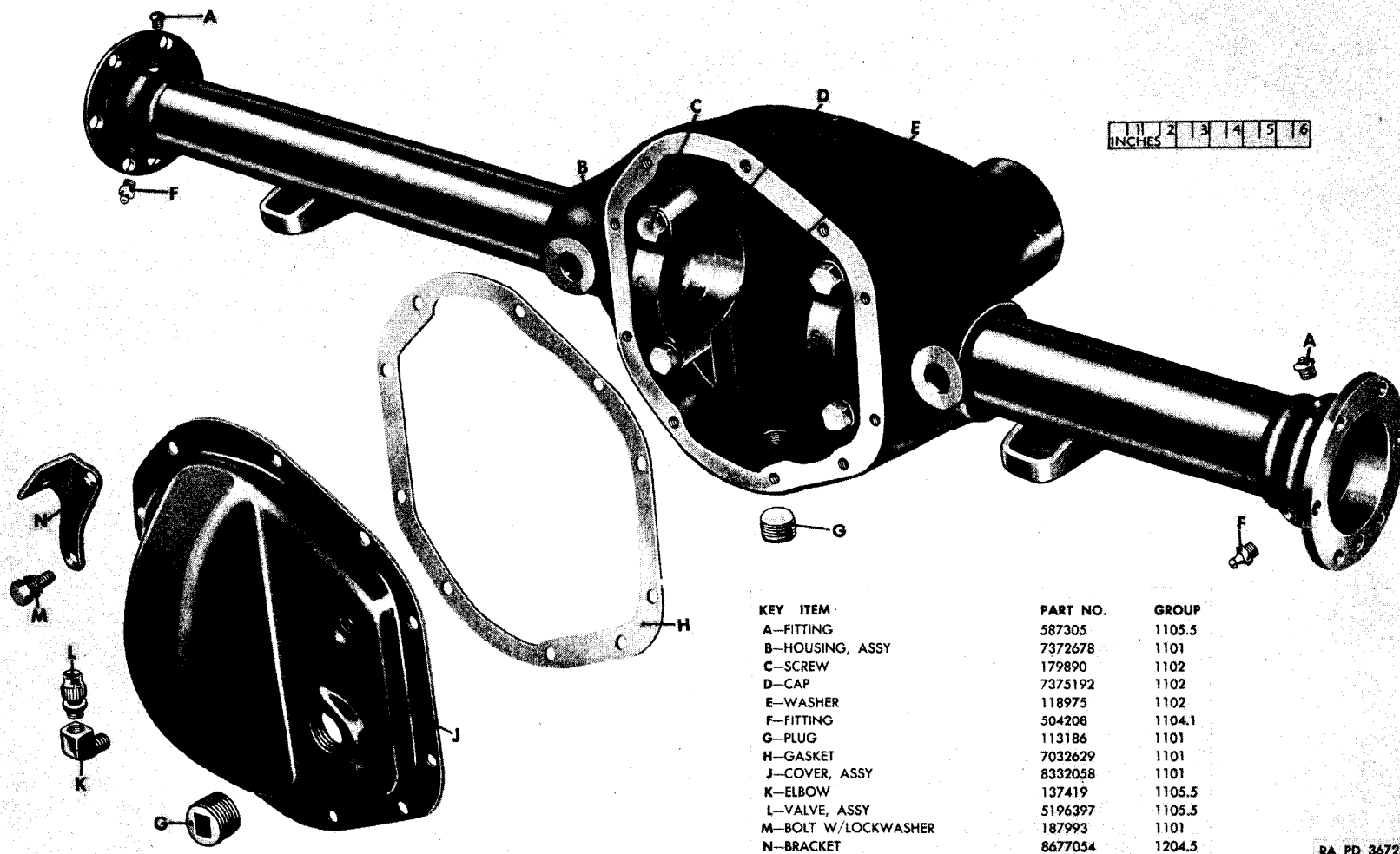
Figure 11-2. Rear axle housing—exploded view
