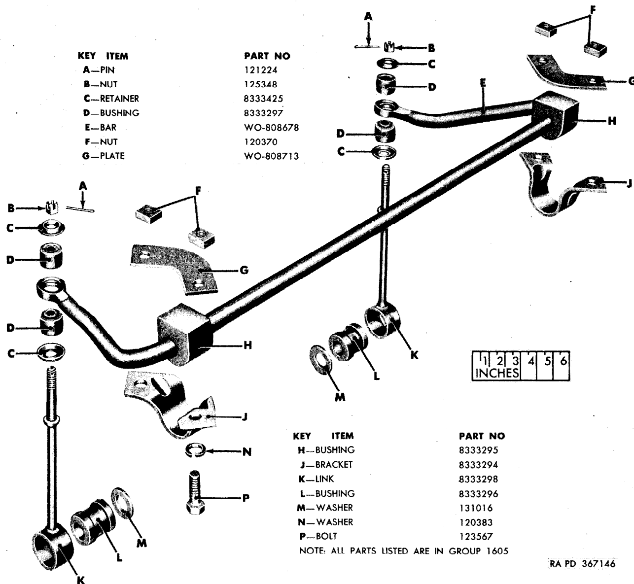
Figure 16-7. Front stabilizer (M170)—exploded view
