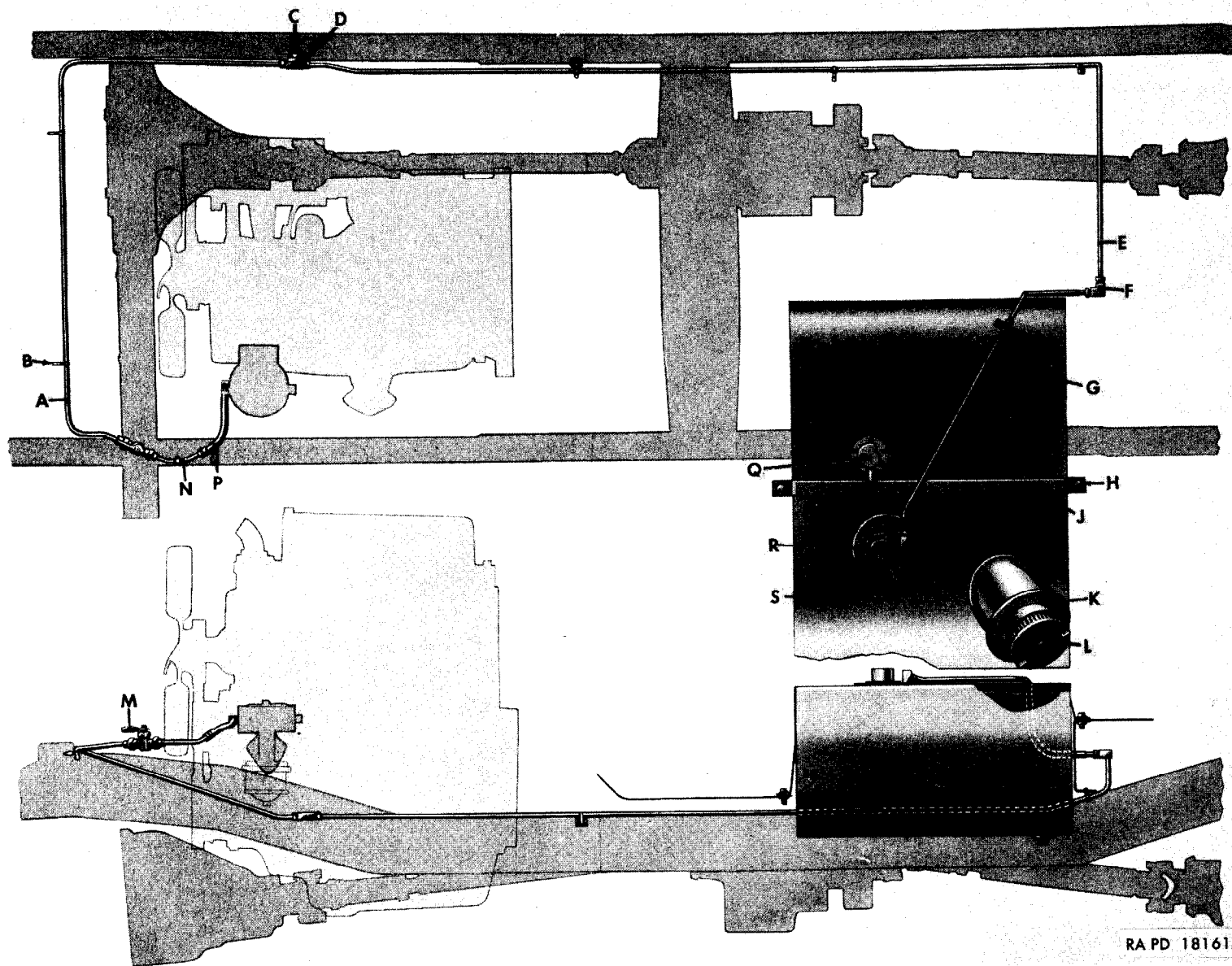
Figure 03-11. Fuel system
