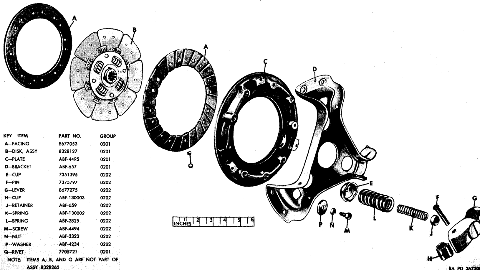
Figure 02-1. Clutch, assy (8328265)—exploded view
