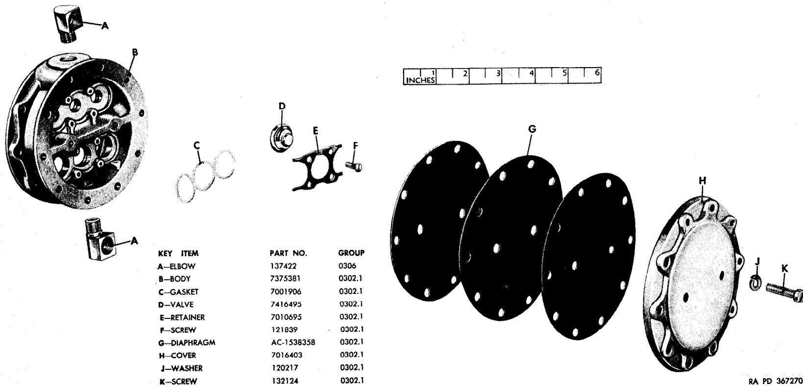
Figure 03-3. Fuel and vacuum pump (fuel section)—exploded view
