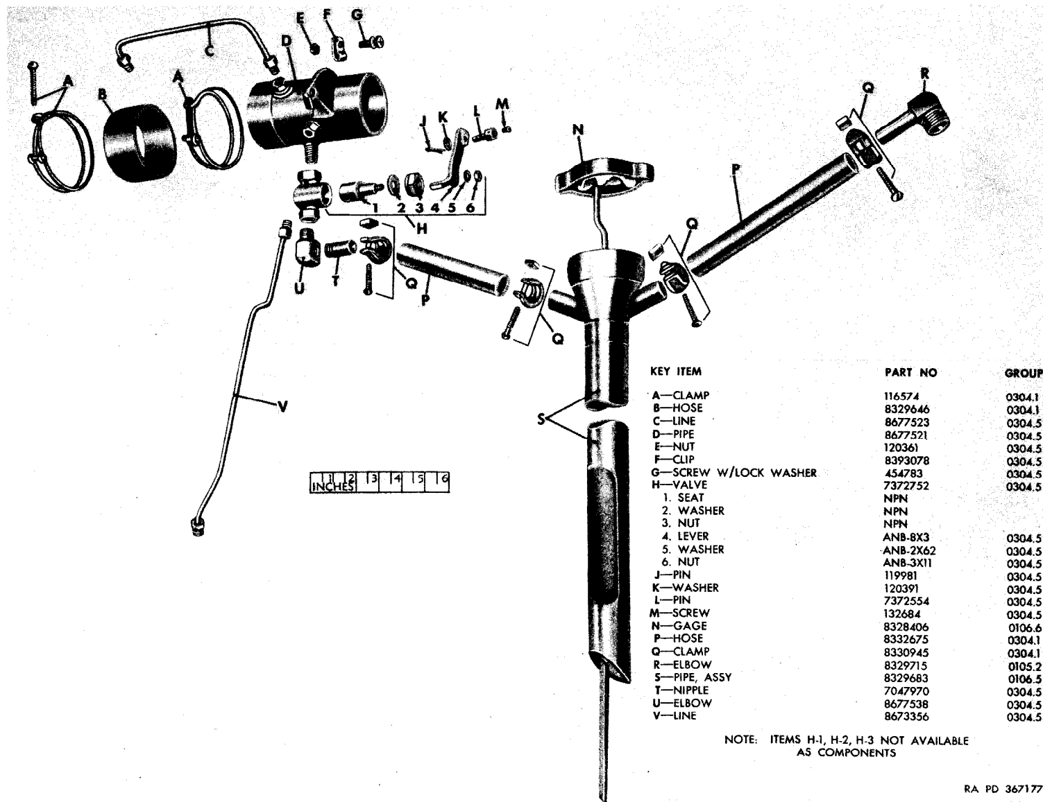
Figure 01-15. Upper vent system—exploded view
